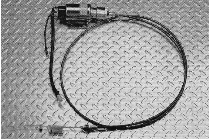
SOLENOID OPERATED CABLE ASSEMBLY FOR MECHANICAL THROTTLES
